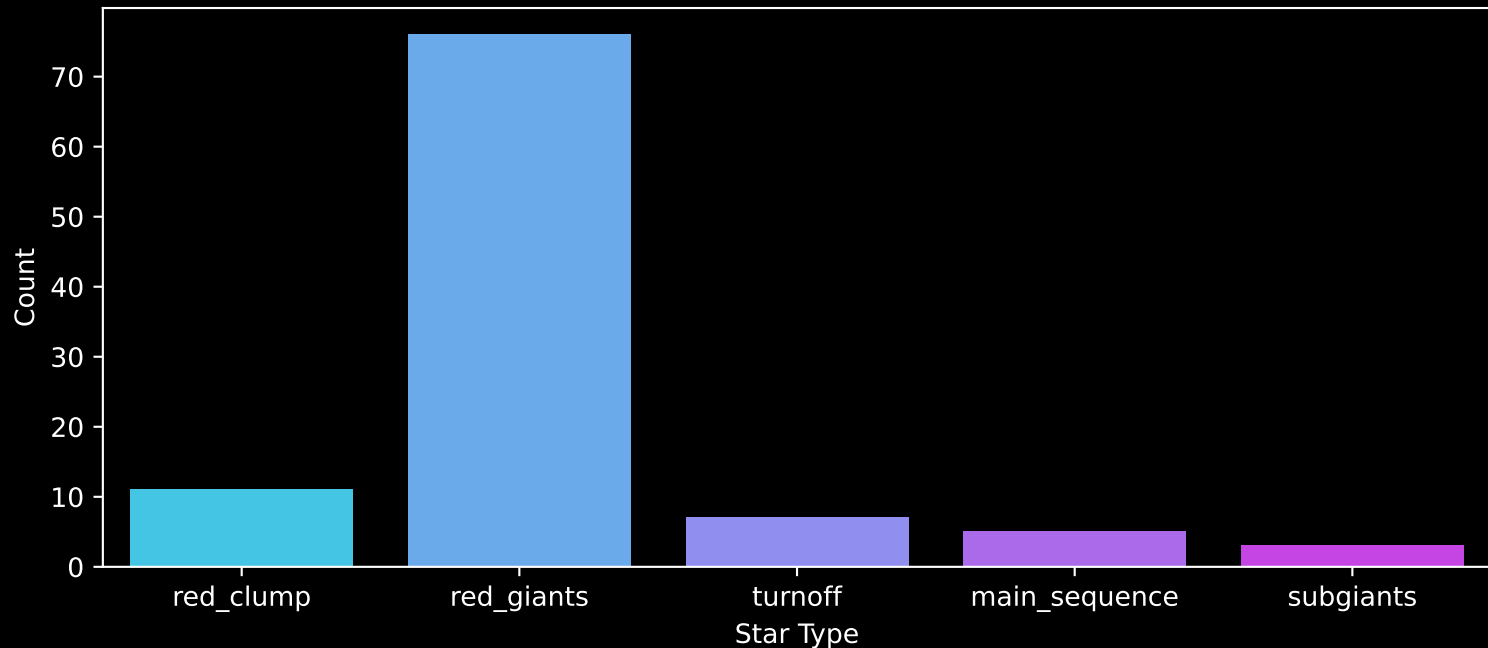
APOGEE DR17 Field: [LMC29] Count plot of Star Type
