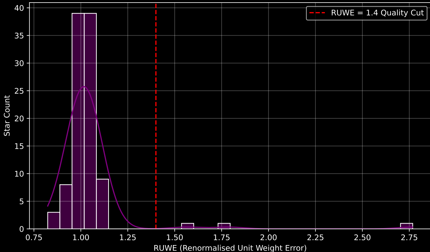
GAPOGEE DR17 Field [LMC29] RUWE Distribution (n= 101)
