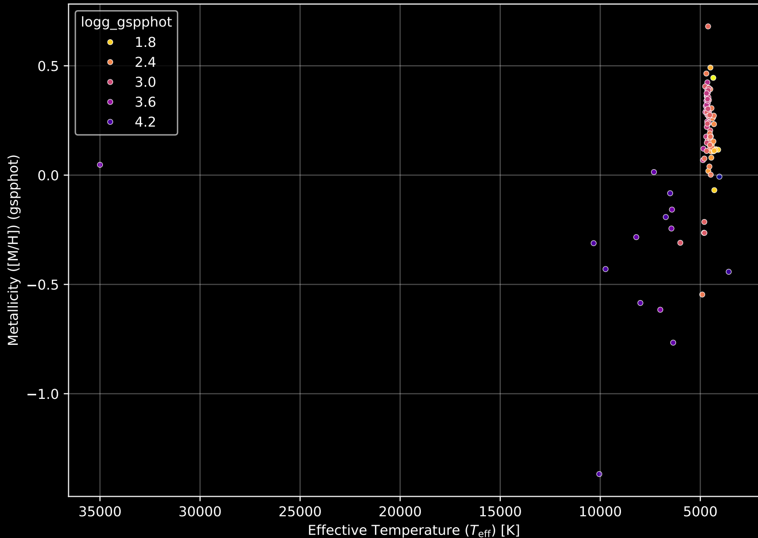
APOGEE DR17 Field: [LMC29] Stellar Population Parameters (n= 102)
