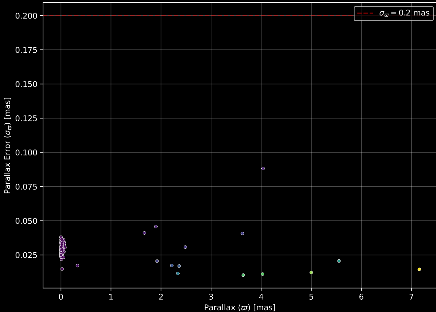
APOGEE DR17 Field: [LMC29] Parallax Quality (n= 102)
