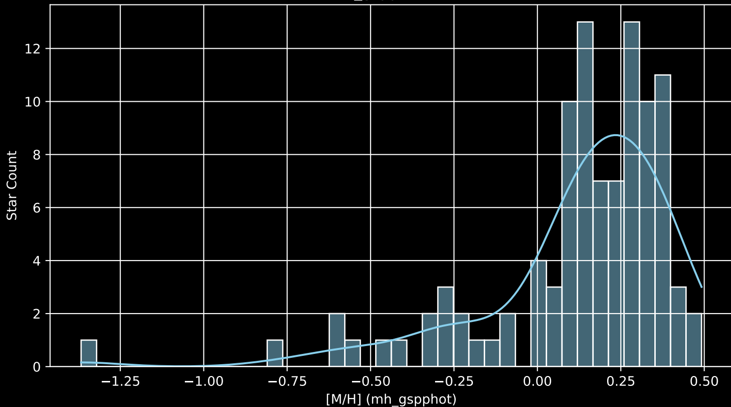
APOGEE DR17 Field: [LMC29 [M/H] (mh_gspphot) (n= 101)
