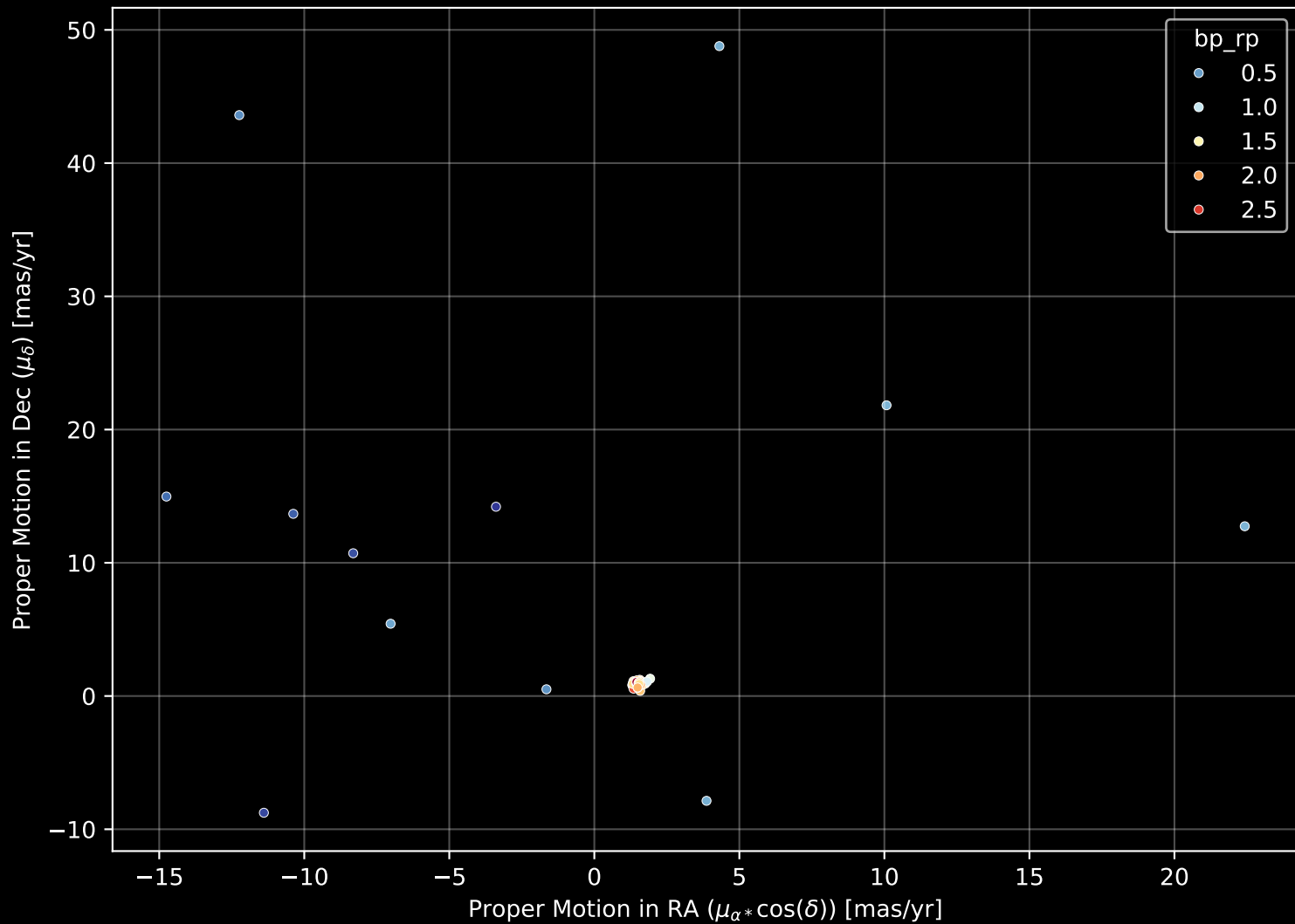
APOGEE DR17 Field: [LMC29] Proper Motion Diagram (n= 102)
