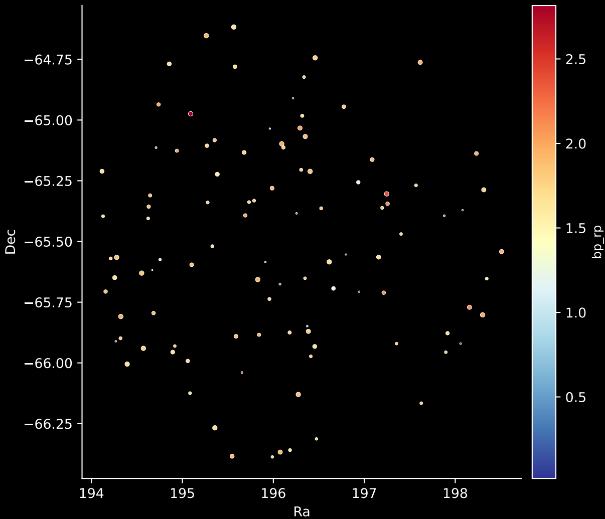
APOGEE DR17 Field: [LMC29] Stars: 102
